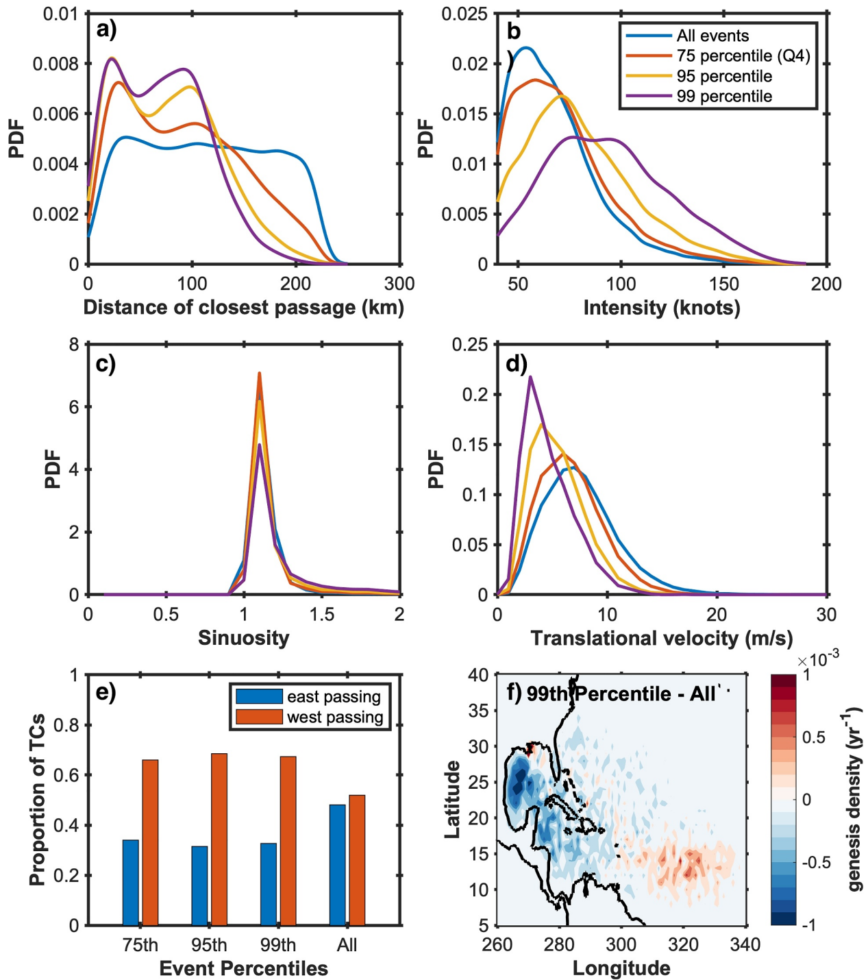
Figure 7. Probability distribution functions of tropical cyclone (TC) distance of closest passage (a), max wind speed (b), sinuosity (c), and translational velocity (d) for fourth quartile (75th percentile) rainfall (red), 95 percentile rainfall (yellow), 99th percentile rainfall (purple) and all (blue) TC events. (e) Histograms of the proportion of 75th, 95th, 99th, and all tropical cyclone precipitation events in the synthetic data set that pass De Soto National Forest to the east (blue bar) versus the west (red bar). (f) Anomaly map of the genesis density for 99th percentile rainfall TC events compared to all TC events.
