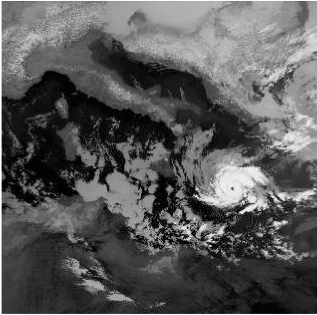
Figure 2. Infrared satellite image of Medicane Celene in the central Mediterranean, at 09:06 UTC 16 January 1995. (Image credit: NOAA, 1995).
