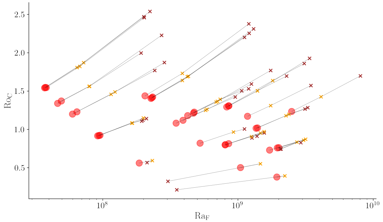
Figure 3.4: Scatterplot of Ro_C vs. Ra_F as in Figure 3.3, with 'x' markers indicating the values at the beginning of each experiment (brown) and at t = 5 rotational periods.
