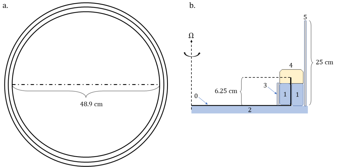
Figure 3.1: Plan view (a) and side view (b) sketches of experimental setup. Numbers in (b) correspond to: 0. Aluminium tank, 1. neoprene foam tape, 2. polystyrene pad, 3. aluminium-foil-lined polyethylene foam, 4. polyurethane-based insulating foam sealant, 5. same as 3., used as a wind barrier.
