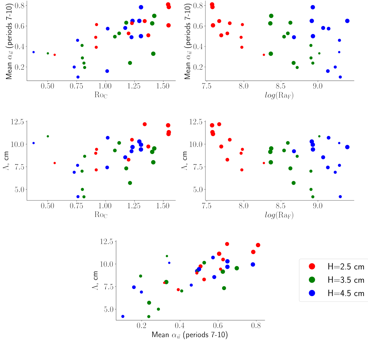
Figure 3.6: Scatterplots comparing the convective Rossby number Ro_C , Flux Rayleigh number Ra_F , two-point correlation length \Lambda , and temporal autocorrelation \alpha for the experiments. The lengths and autocorrelations correspond to the mean value between 7 and 10 rotational time periods. Each marker size is scaled by the rotational period of the experiment (values of 35, 70, 104, 125 or 153 seconds).
