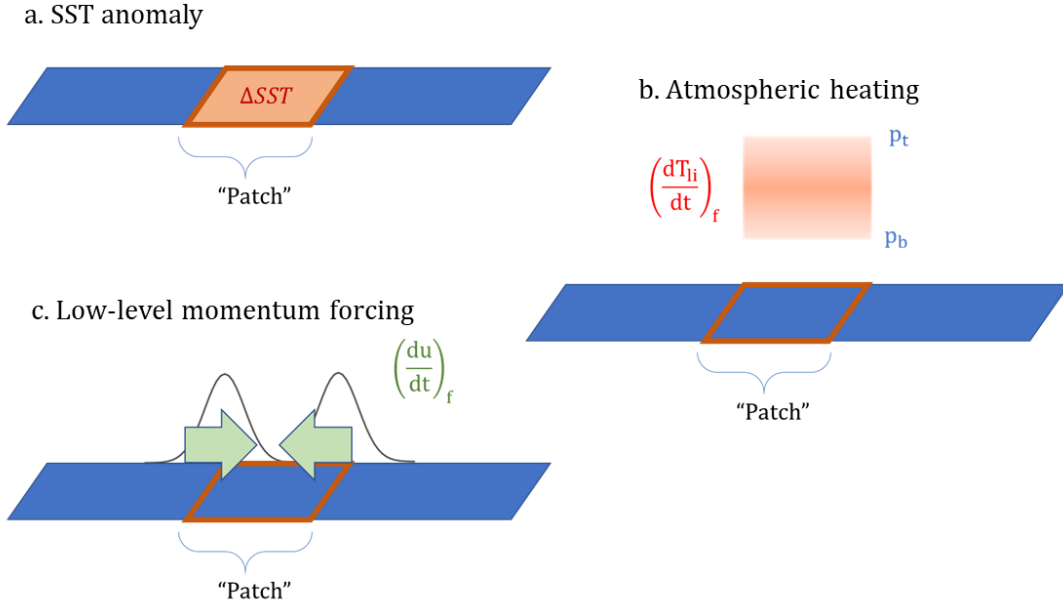
Figure 4.1: Sketches of the setups representing the three different forcings: a. Sea-surface temperature anomaly, b. Atmospheric heating between levels p_b and p_t , c. Low-level momentum forcing. The reference patch for which averages are calculated is indicated in red; geometry is not to scale.
