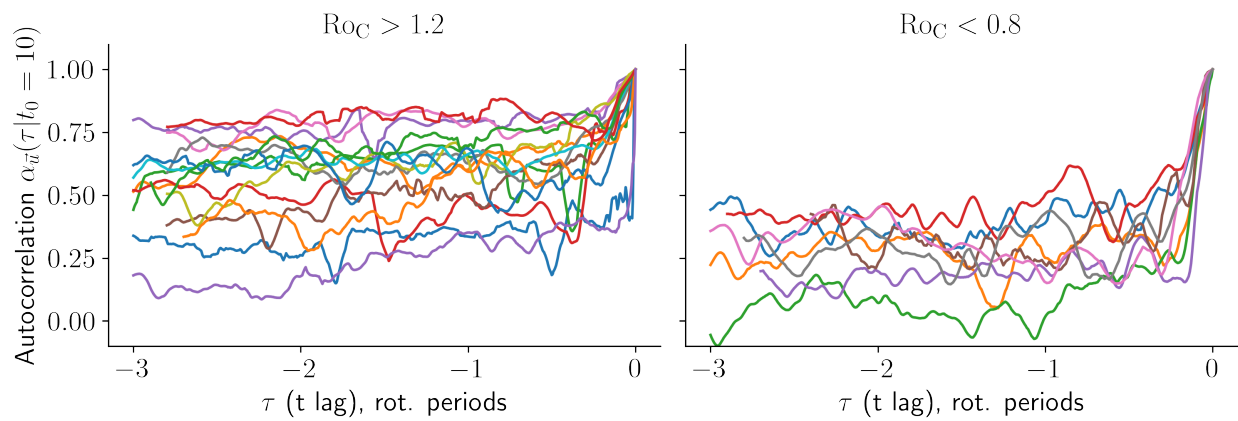
Figure 3.5: Time series of temporal autocorrelation of \vec{u} at t_0 = 10 rotational periods, for experiments with Ro_C > 1.2 (left) and Ro_C < 0.8 (right). The series are smoothed with a forward rolling mean with window size 0.1 for \tau < -0.1 , and a size of \tau for \tau \geq -0.1 .
