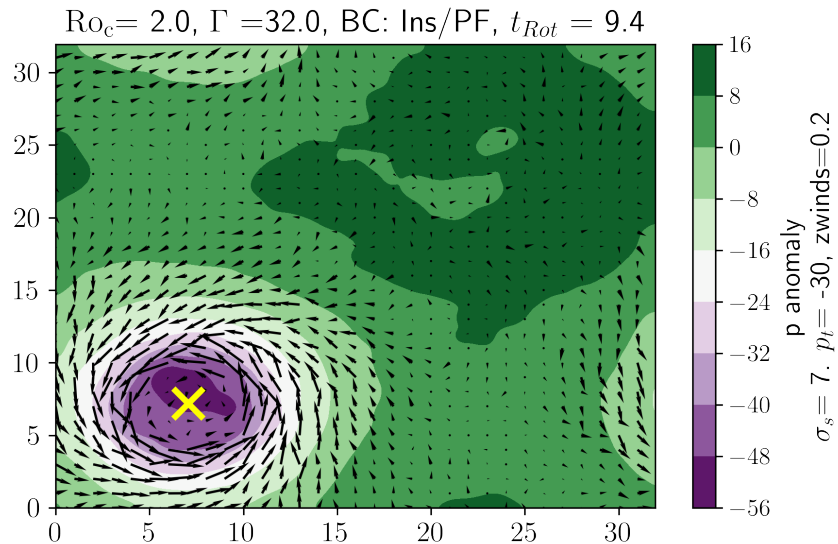
Figure A.5: Plan view of pressure anomaly field and quiver plot of horizontal winds at 20 percent of domain height for simulation with \Gamma = 32 , and convective Rossby number Ro_c = 2.0 after equilibration. A yellow “x” marks the centroid of the low pressure anomaly feature.
