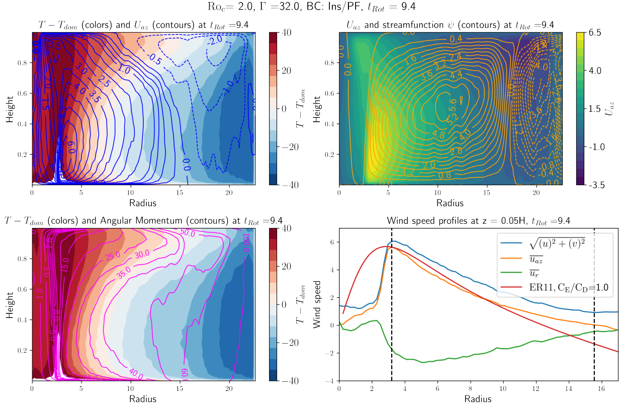
Figure A.8: Contour plots of azimuthally averaged quantities (temperature anomaly with respect to domain mean, azimuthal wind speed, angular momentum, Stokes streamfunction), and azimuthally averaged wind speed profile of vortex formed in domain with aspect ratio 32 and convective Rossby number Ro_C = 2.0 .
