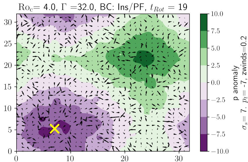
Figure A.7: Same as A.5 but with Ro_c = 4.0 .
