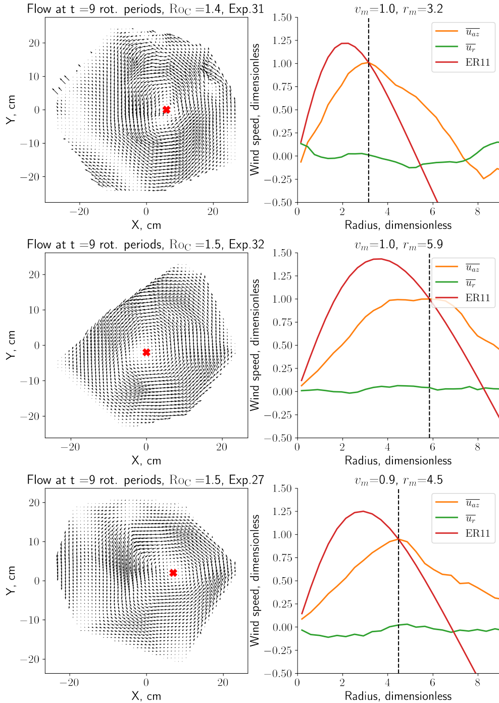
Figure 3.7: Flow field (left) and azimuthally-averaged wind profile at vortex center for select experiments with persistent, large-scale cyclones (right). The azimuthal wind speeds are in orange, the radial winds are in green, and the azimuthal wind based on the model by Emanuel and Rotunno, 2011 with C_E/C_D = 1 is denoted in red. The maximum azimuthal wind speed v_m and the radius of maximum wind r_m and indicated in the title, and the latter is marked with black dashed lines.
