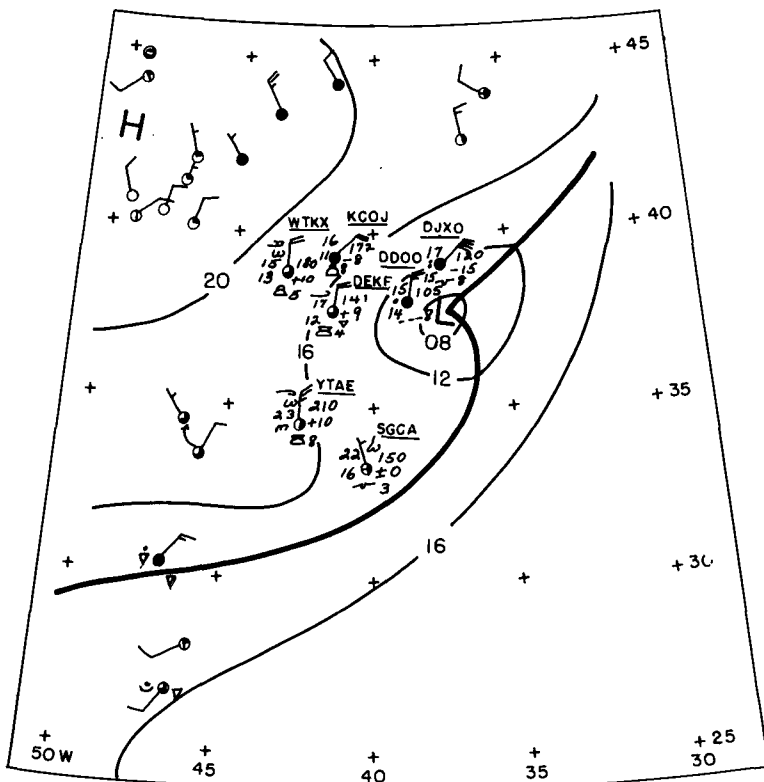
FIG. 4. As in Fig. 1 except for 1800 GMT.
