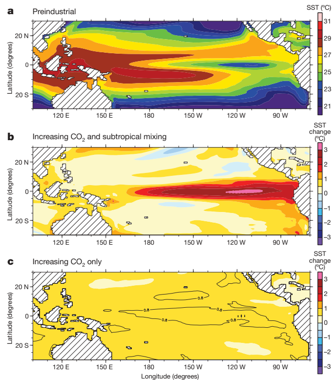
Figure 4 | SST changes in the tropical Pacific simulated by the coupled model. a , SSTs for preindustrial climate conditions; b , SST changes in response to increasing \text{CO}_2 concentration from 290 p.p.m. (preindustrial) to 355 p.p.m. (the level of 1990) and increasing vertical diffusivity in the upper ocean (0–200 m) in the extra-tropical bands ( 8^\circ – 40^\circ north and south of the Equator), after 200 years of calculations for the Pliocene scenario. The SST increase has a clear signature of permanent El Niño-like conditions, with the warming reaching 3.5^\circ \text{C} in the eastern equatorial Pacific. c , SST changes in response to increasing \text{CO}_2 concentration alone. The SST increase is virtually uniform and remains below 1^\circ \text{C} .
