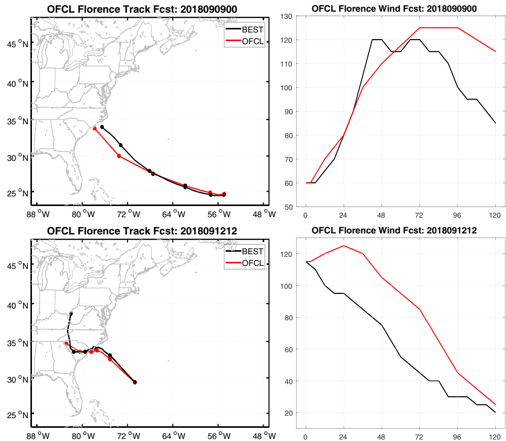
Figure 1. The official 120-hr position (left) and intensity forecasts (knots) of Hurricane Florence issued by the National Hurricane Center at 00Z 9 (top) and 12Z 12 (bottom) September 2018, corresponding respectively to about 5 days and 36 hr before its actual landfall.
