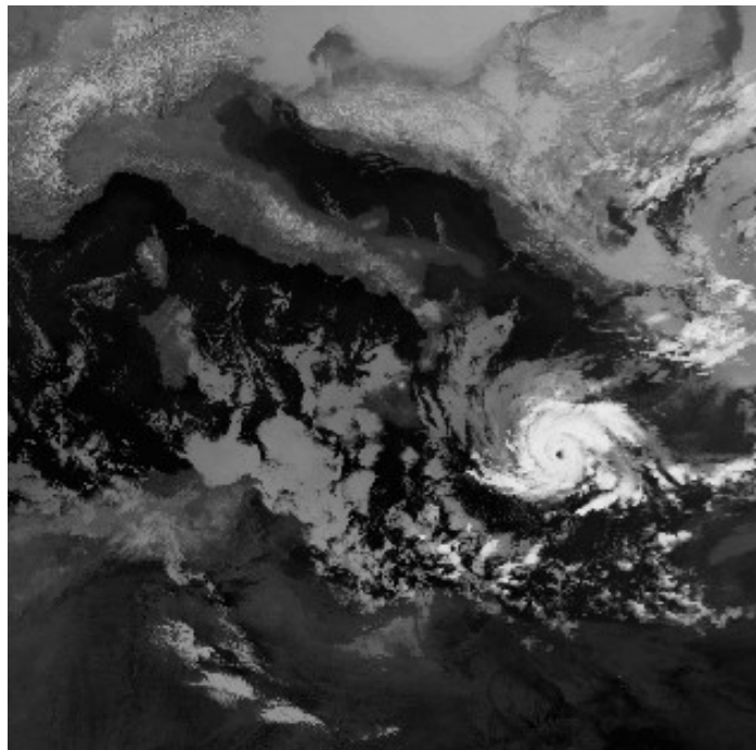
Figure 2: Infrared satellite image of Medicane Celeno in the central Mediterranean Mediterranean , at 09:06 UTC 16 January 1995.
