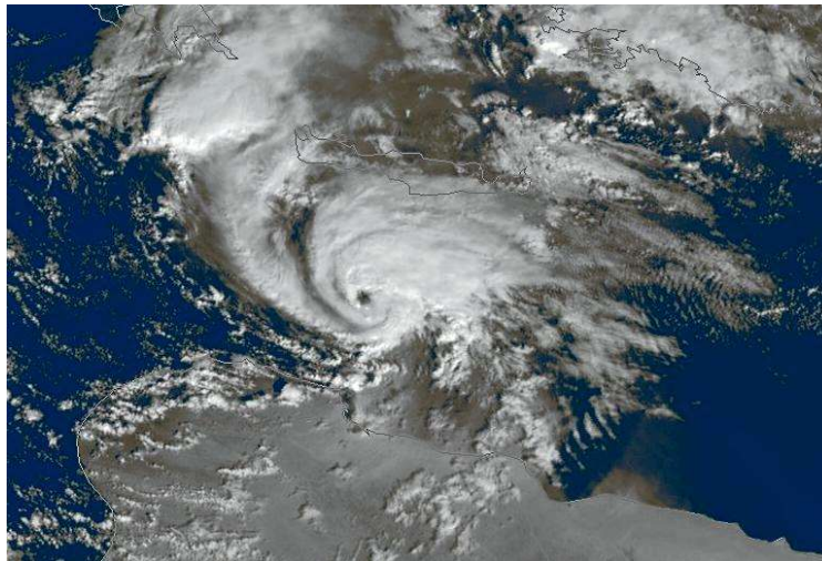
Figure 6: Mediane between Crete and Libya on 15 December 2005.
