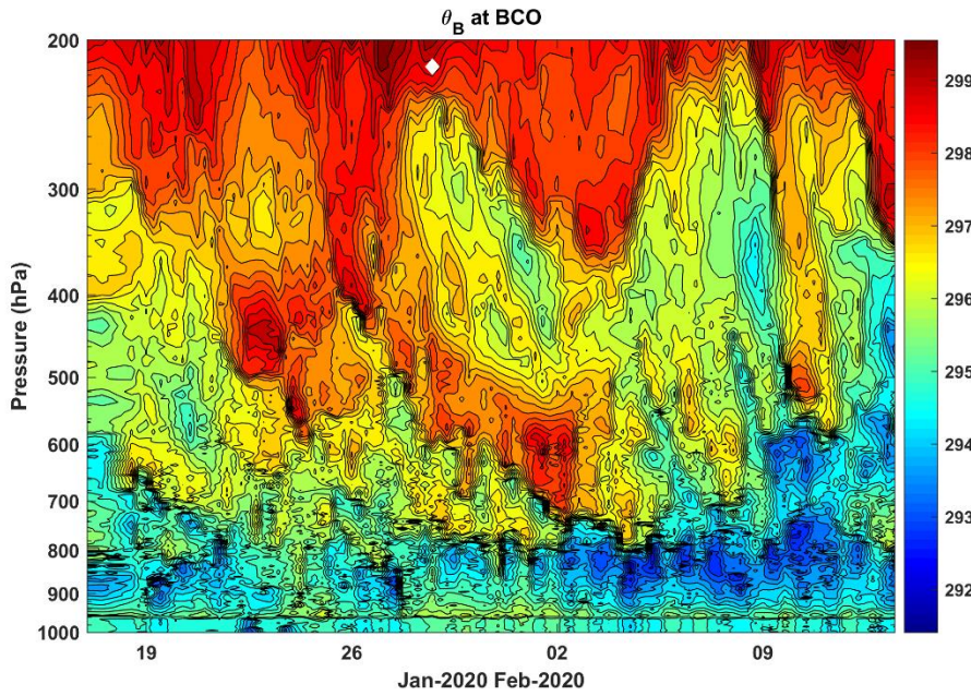
Buoyancy potential temperature (Temperature of just saturated air at 960 hPa such that when reversibly lifted, its density temperature is the same as the environment at the indicated level)
