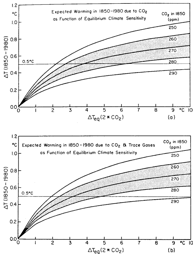
Fig. 17. Computed global warming between 1850 and 1980 as a function of the equilibrium climate sensitivity for doubled CO 2 (315 ppm → 630 ppm), \Delta T_{eq}(2*CO_2) . Results are shown for five values of the assumed abundance of CO 2 in 1850; the shaded area covers the range 270±10 ppm recommended by WMO (1983). (a) includes only CO 2 growth, while (b) also includes the trace gas growths of Table 4. In all cases CO 2 increases linearly from the 1850 abundance to 315 ppm in 1958 and then according to measurements of Keeling et al. (1982).
