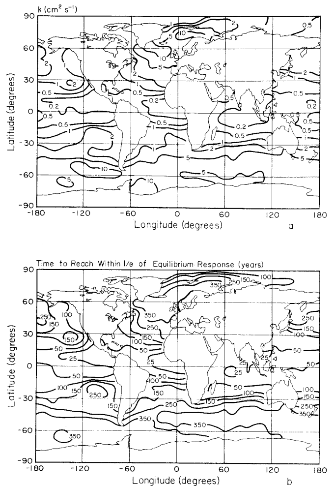
Fig. 15. (a) Geographic distribution of effective thermocline diffusion coefficient, k ( \text{cm}^2 \text{ s}^{-1} ). k is derived from Eq. 25 and the global distribution of N^2 , the latter obtained from the ocean data of Levitus (1982). (b) Geographic distribution of the 63 percent response time for surface temperature response to doubled \text{CO}_2 in the atmosphere. Only geographic variability of k and mixed layer depth are accounted for. \Delta T_{\text{eq}}(2 \times \text{CO}_2) is taken as 4.2^\circ\text{C} everywhere. The flux into the ocean is from Eq. (24).
