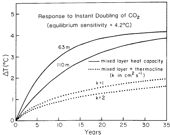
Fig. 16. Transient response to step function doubling of atmospheric \text{CO}_2 from 315 ppm to 630 ppm, computed from (24) with three representations of the ocean. The 63 m mixed layer corresponds to the mean mixed layer depth in the 3-D experiments; 110 m is the global-mean annual maximum mixed layer depth obtained from global ocean data. The curves including diffusion beneath the mixed layer are not exponentials (Appendix A).
