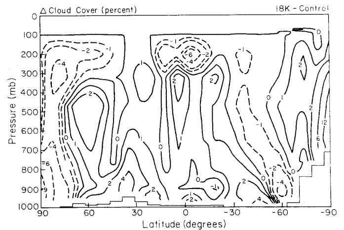
Fig. 11. Cloud cover for the 18K simulation and differences with the control run. The control run is described in detail in paper 1.
