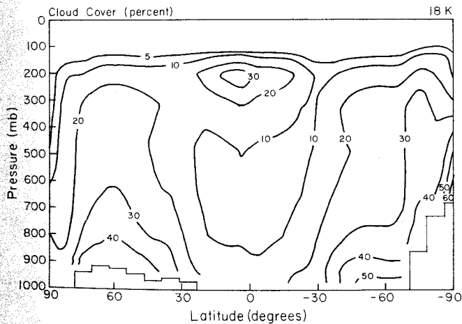
Fig. 11. Cloud cover for the 18K simulation and differences with the control run. The control run is described in detail in paper 1.
