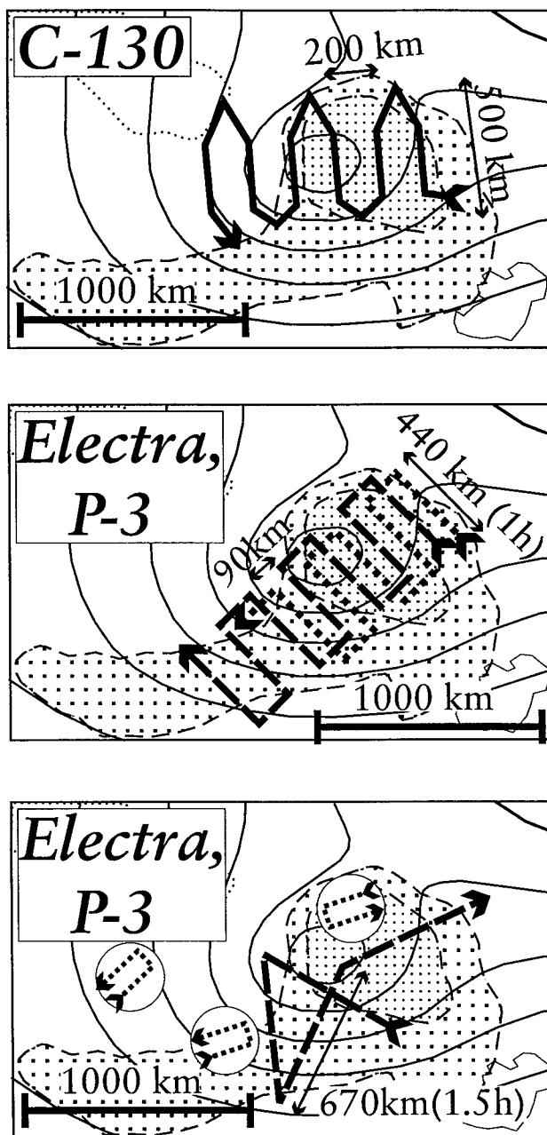
FIG. 9. Schematics of system-relative flight patterns to be employed by the turboprop aircraft in the MSA. The flight tracks are overlaid on the new composite structure for the type 1 frontal wave rederived from automatic tracking and automatic classification of trajectories covering the mature stage. The solid lines are surface pressure, and the shaded areas represent upward vertical velocity at 700 mb. The dotted line denotes an area of descent. The top panel shows the UKMO C-130 pattern going toward the clear air, low tropopause, part of the cyclone. The two other panels show the two main alternatives for the NCAR Electra (dotted track) and NOAA P-3 (dashed track). The middle panel shows the so-called "lawnmower pattern" from which an overall observation of the ascent zone will be derived. The lower panel shows the overall exploration of the wave by the P-3, while circles mark possible areas where the Electra could perform mesoscale sampling of rainbands and other structures. (Objective composite frontal wave is courtesy of Franck Ayrault.)
