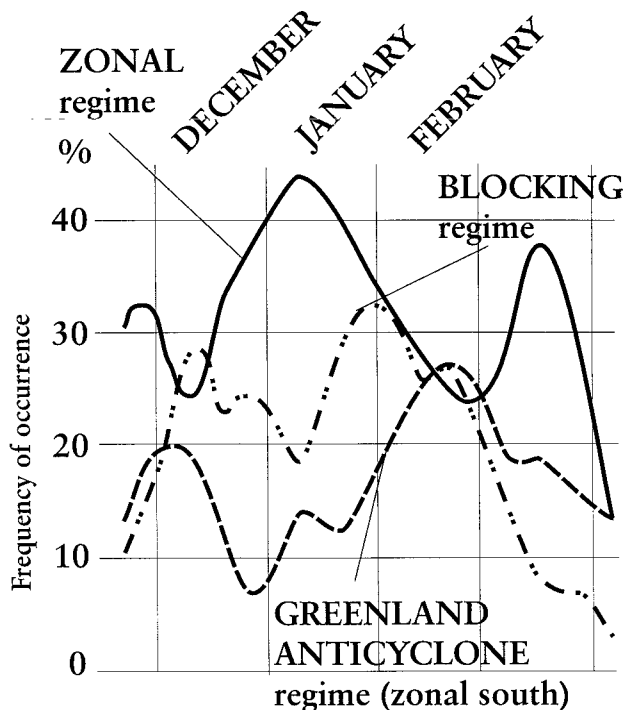
FIG. 3. Climatological frequency of weather regimes over the North Atlantic during the winter months. Derived from ECMWF analyses from 1986 to 1994. The onset of the zonal or of the Greenland anticyclone regimes implies cyclogenesis events for FASTEX, unlike the blocking regime. (Courtesy of Franck Ayrault.)
