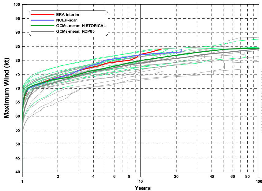
FIG. 7. Return period (yr; horizontal axis) of NA polar lows according to the maximum wind induced at the surface (kt; vertical axis) calculated from the reanalyses and from the set of BEST GCMs (multimodel mean; historical and RCP8.5 scenarios; see legend; individual models also shown as thin lines). Model consensus on the present-to-future sign of change at 66% and 80% levels is indicated along the right side of the figure.
