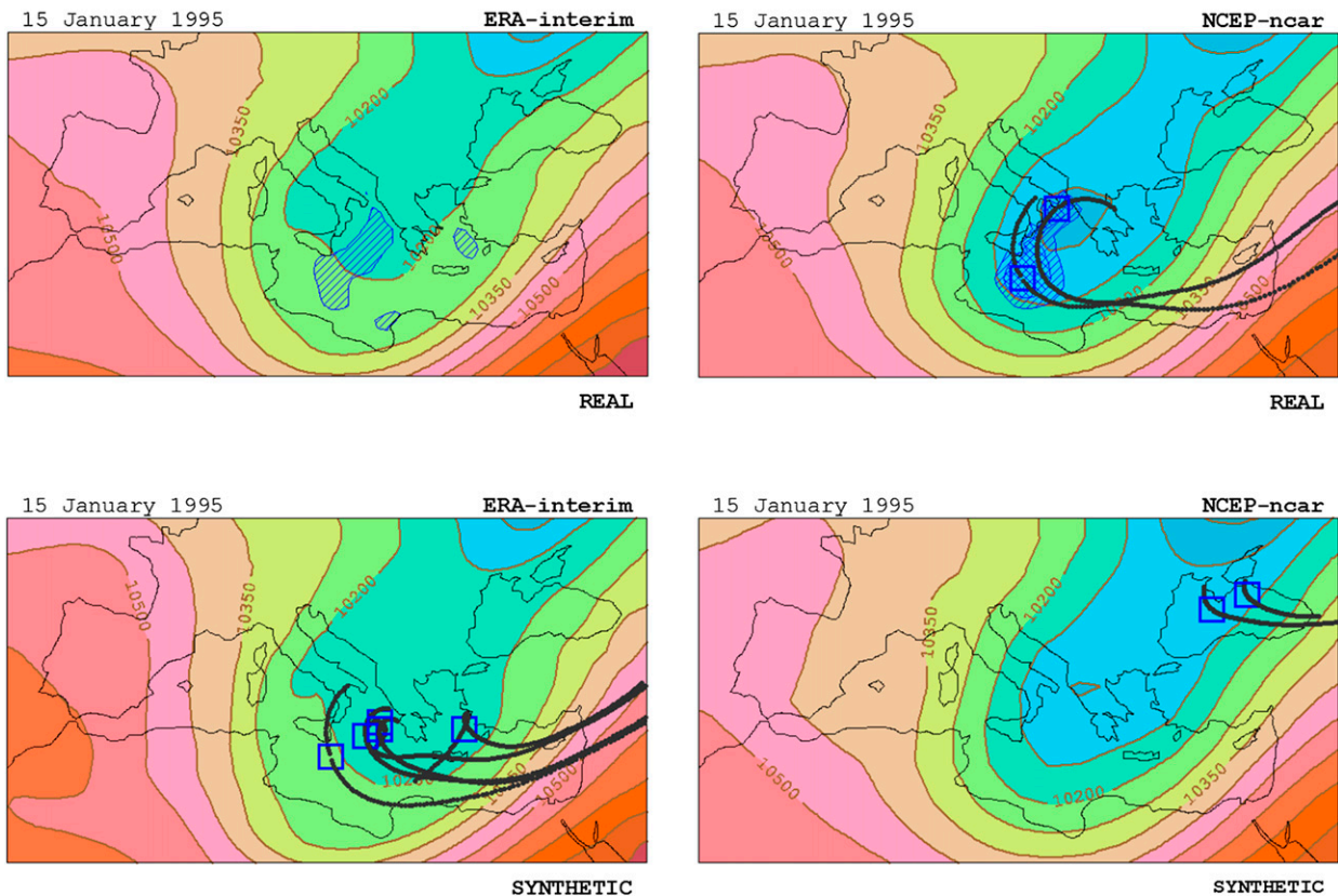
FIG. 2. Synoptic scenario corresponding to the “Libyan” medicane [(top) Meteosat IR channel satellite image indicates the position of the storm at 1200 UTC 16 Jan 1995]. Shown here are the daily average on 15 Jan of geopotential height at 250 hPa (contour interval 75 gpm) extracted (middle) from the ERA-Interim and NCEP–NCAR reanalyses (REAL) and (bottom) from a synthetically generated analog for each reanalysis (SYNTHETIC). For each case, potential tracks identified during the episode according to the method described in the text are indicated, where the blue square on each track indicates the storm genesis location (see text). For the reanalyses, the daily average of the GEN index is also indicated (hatched area above 5 units of the index; cross-hatched area above 10 units). (Note that ERA-Interim did not produce tracks.)
