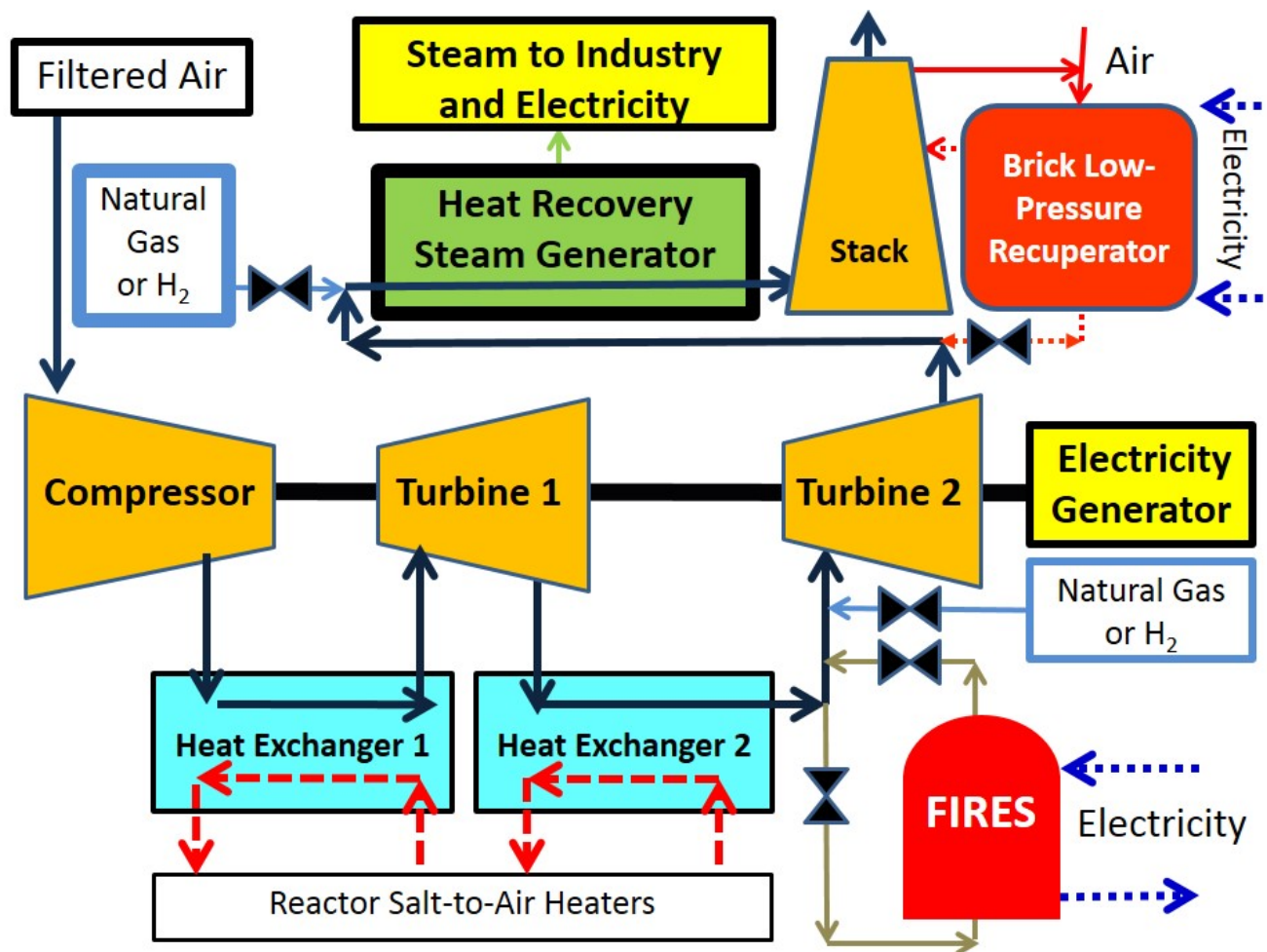
Fig. 2.12. NACC with Heat Storage and Use of Auxiliary Fuels (Natural Gas, Hydrogen, Stored Heat [FIRES and Brick Recuperator], Other).
