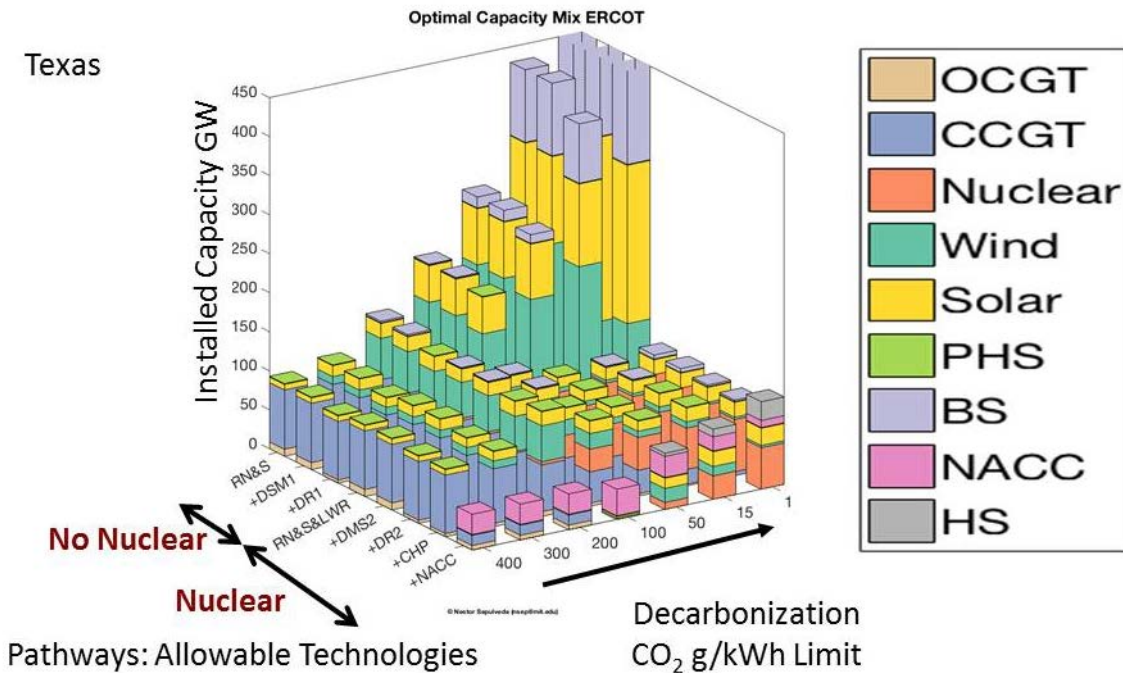
Fig. 4.2. Optimal 2050 Texas Installed Capacity vs. Added Technologies and CO 2 Limits
