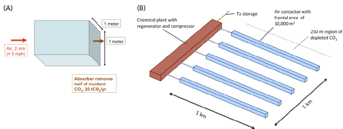
Figure 1.2. Schematic representations of A) a 1 \text{m}^2 intake area contactor capturing 20 \text{tCO}_2/\text{yr} , and B) a facility for capturing 1 \text{MtCO}_2/\text{yr} . The facility in B consists of five structures, each 10 meters high and 1 km long, and could collect 1 \text{MtCO}_2/\text{yr} if air passed through at 2 m/s and 50% of the \text{CO}_2 were collected. The structures are spaced 250 meters apart, and the footprint of the system is roughly 1.5 \text{km}^2 . Approximately six of these systems would be required to compensate for the emissions of a 1 GW coal plant. Buildings not to scale.
