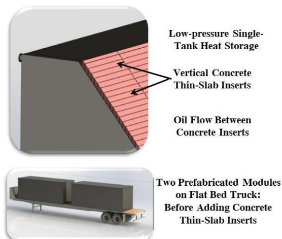
Fig. 2.5. Westinghouse Thermal Heat Storage Module for 1 MWh of Electricity Storage
