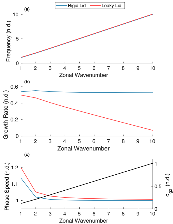
FIG. 1. Non-dimensional (a) frequency, (b) growth rate, and (c) phase speed and for the fastest-growing v = 0 mode. Vertical group velocity of the leaky mode is shown in black in (c), while rigid-lid solutions are shown in blue and leaky-lid solutions shown in red. Non-dimensional parameters are \alpha = 1.5 , \chi = 0.5 , C = 0 , \gamma = 2 , D = 0.5 , G = 0.1 , and S = 100 .
