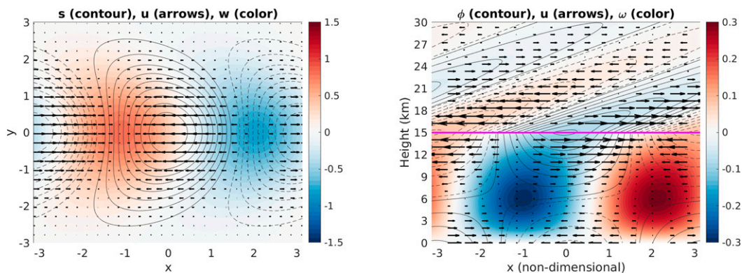
FIG. 2. Eigenfunction of the v = 0, k = 1 mode corresponding to the parameters detailed in Fig. 1, on (left) a horizontal cross section at the surface and (right) a vertical cross section centered on the equator. Contours indicate the saturation entropy or geopotential, where solid (dashed) lines indicate positive (negative) perturbations. Arrows indicate zonal velocity perturbations, and color shading indicates vertical velocity or \omega perturbations, where indicated. Magenta line outlines the tropopause.
