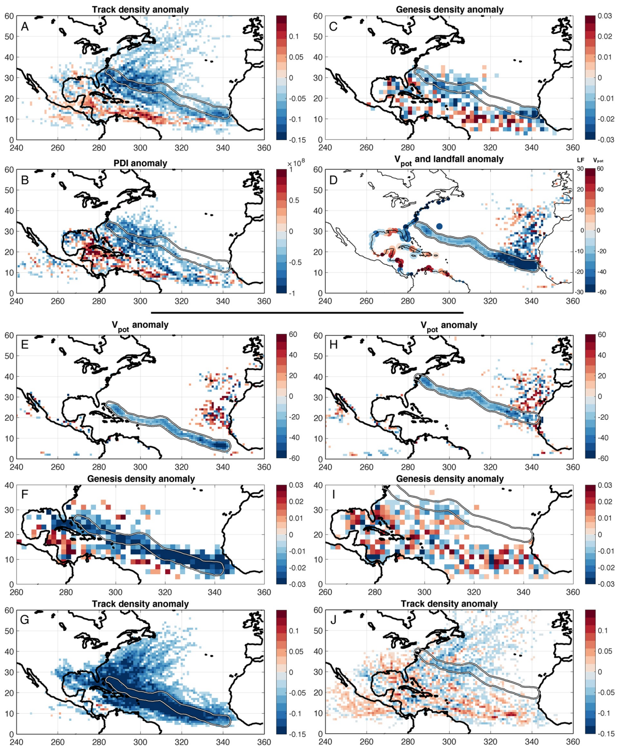
Figure 3. Anomaly maps for (a) Track density (TCs per 1^{\circ} grid cell per year), (b) Power dissipation index (PDI; \text{m}^3 \text{s}^{-2} ), (c) Genesis density (TCs per 2^{\circ} grid cell per year), and (d) Potential intensity ( V_{pot} ; knots) and landfall frequency anomaly (bubbles along the North and South American coastline; % change). Landfall bubble size is proportional to the annual number of landfalls per year in the control simulation. (e)–(g) Potential intensity anomaly (knots), genesis density anomaly (TCs per 2^{\circ} grid cell per year) and track density anomaly (TCs per 1^{\circ} grid cell per year) for the Florence-South wake. (h)–(j) as in (e)–(g) but for the Florence-North wake. All anomalies are relative to the control simulation. The -0.5^{\circ}\text{C} SST anomaly isotherm of the applicable wake is contoured on each panel for reference.
