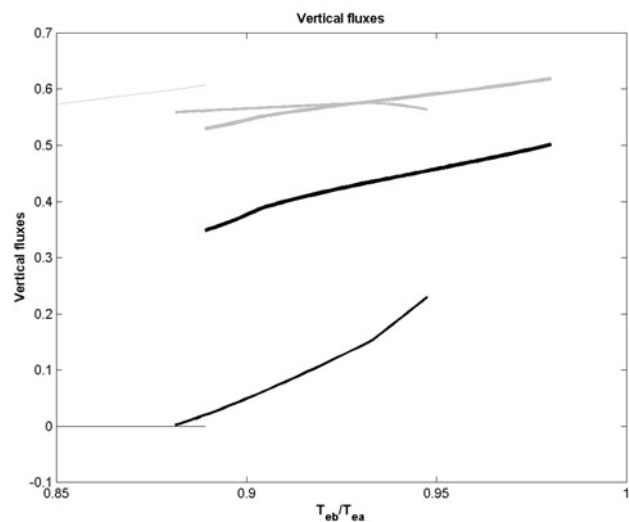
Figure 5. As in 2, but showing turbulent vertical fluxes in the low-latitude box. Gray lines show fluxes from level 1 to level 2; black lines show surface fluxes.
