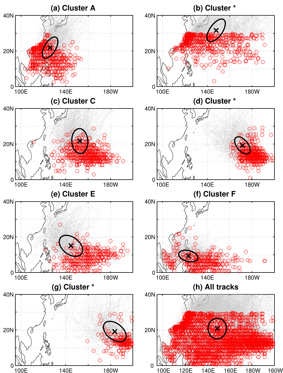
Figure 4. Western North Pacific model tracks in individual clusters for CMIP5 model M12 in the historical simulation. Model clusters that do not correspond to any of the observed clusters are marked with an asterisk (*).
