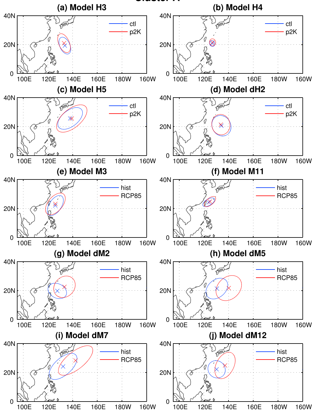
Figure 9. Track ellipses in cluster A for selected models that have a statistically significant increase in the variance of Y , for (a–d) HWG and (e–j) CMIP5 models.
